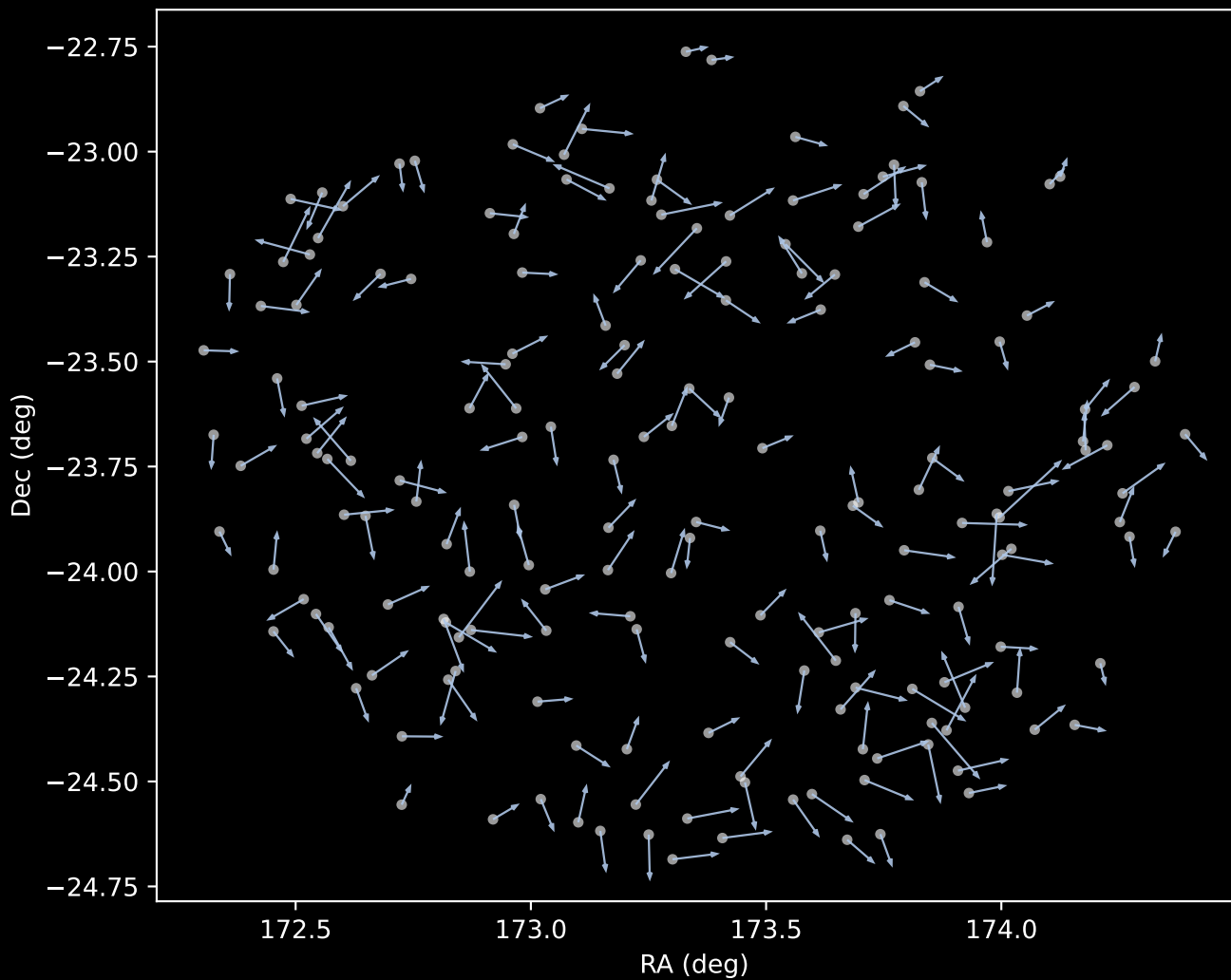
GALAH DR4 Cluster 1 Proper Motion Vectors (n=180)
