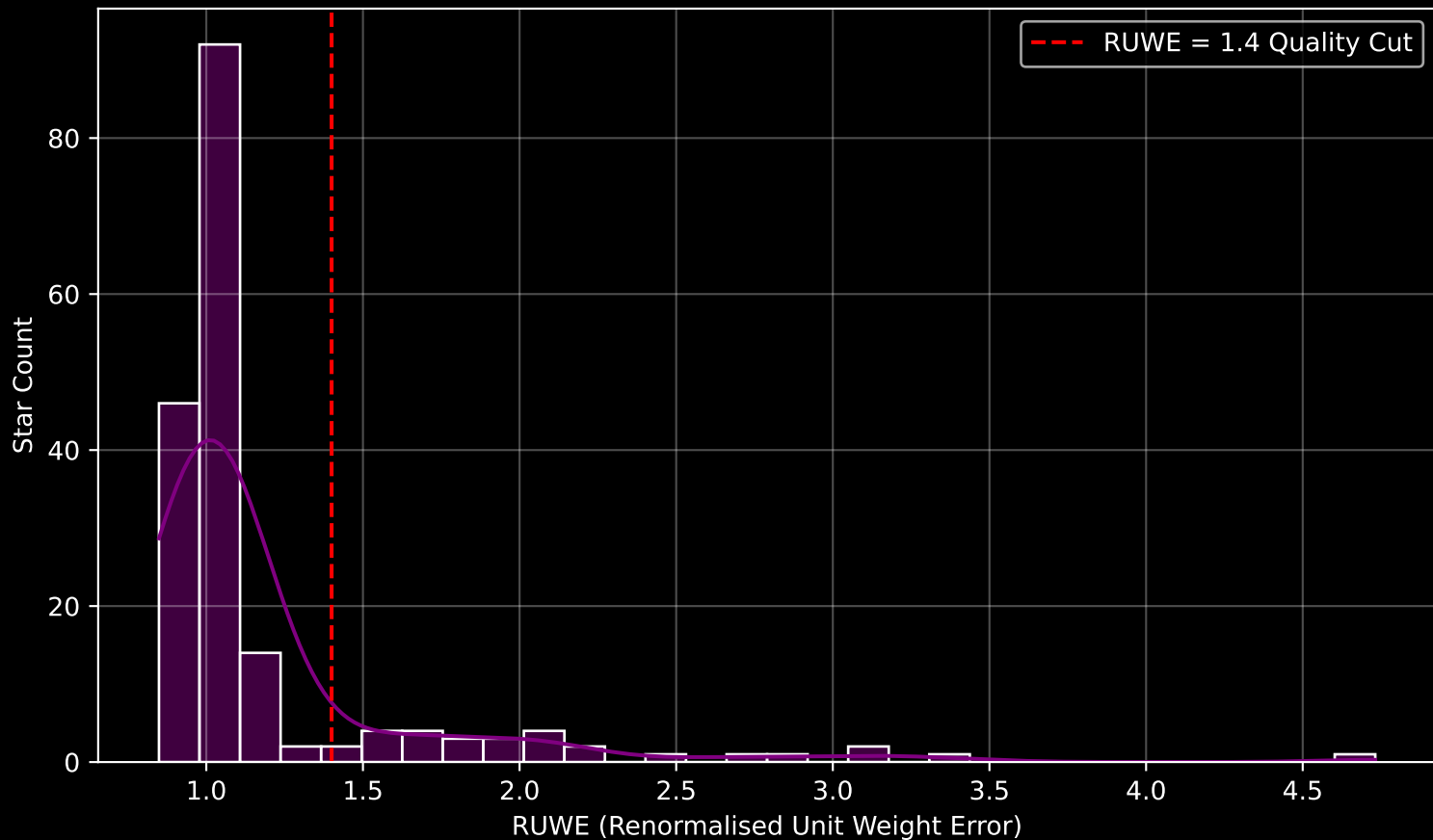
GALAH DR4 Field [507] RUWE Distribution (n= 183)
