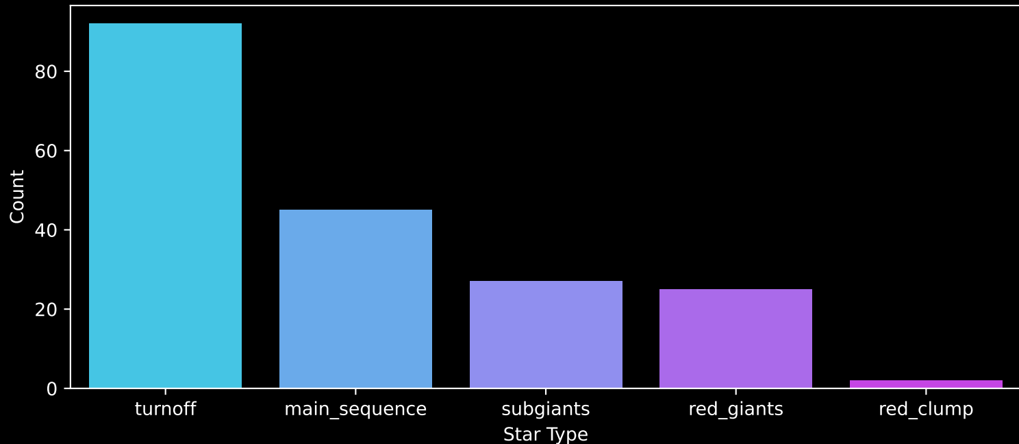
GALAH DR4 Field: [507] Count plot of Star Type
