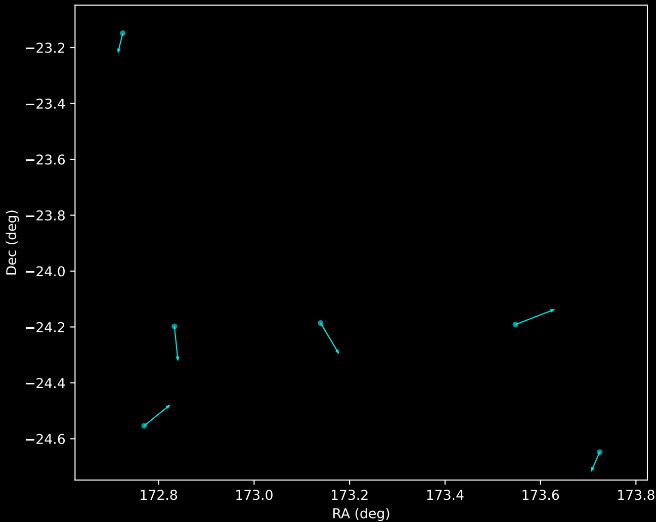
GALAH DR4 Noise Stream Proper Motion Vectors (n=6)
